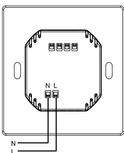
Figure 7. Wiring
