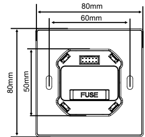
Figure 3. Dimensions - Front View
