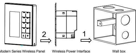
Figure 8. Installation
