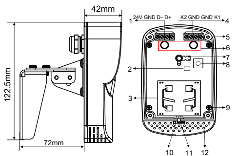
Figure 4. Dimensions - Side View
