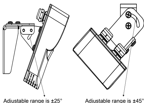
Adjustable range is \pm 25^\circ Figure 6. Adjustable range upwards and downwards
