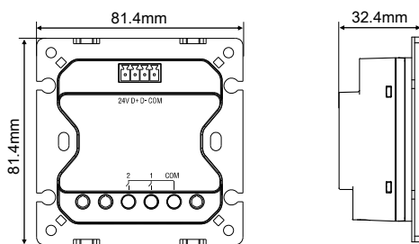
Figure 3. Dimensions - Back View
