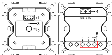
Figure 5. Components - Front View
