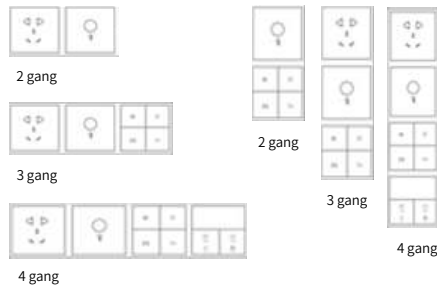
Figure 12. Horizontal installation
