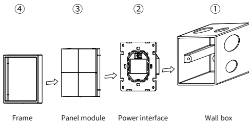
Figure 11. Installation
