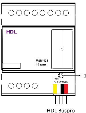
Figure 4. Components - Front View
