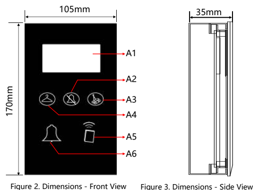
Figure 2. Dimensions - Front View
