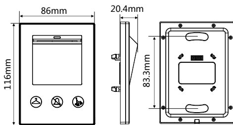
Figure 6 - 8. Dimensions HDL-MPTC03.46
