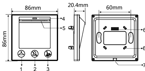
Figure 3 - 5. Dimensions HDL-MPTC03.48
