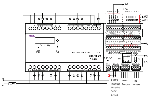
Figure 4. Wiring
