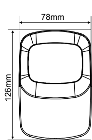
Figure 2. Dimensions-Front View
