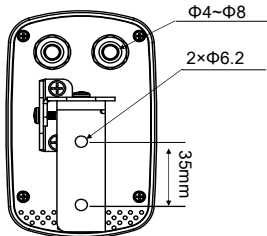
Figure 4. Dimensions-Back View
