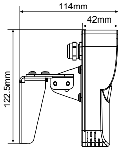
Figure 3. Dimensions-Side View
