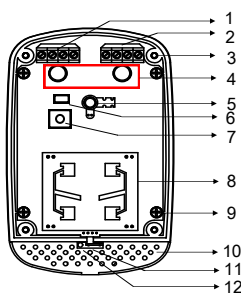
Figure 7. Interior View
