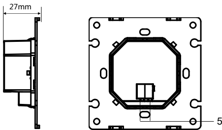
Figure 3. Dimensions - Side View
