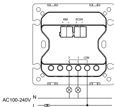
Figure 7. Wiring
