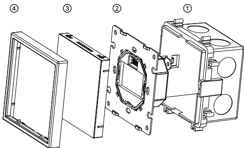
Figure 6. Installation
