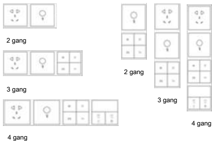
Figure 7. Horizontal installation
