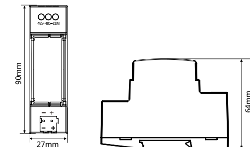
Figure 5. Base - Front View
