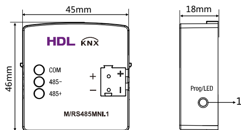
Figure 3. Dimensions - Front View Figure 4. Dimensions - Side View
