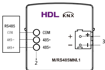
Figure 7. Wiring
