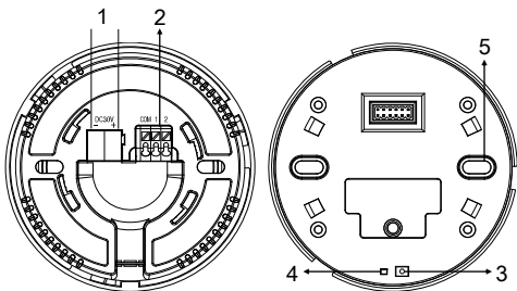
Figure 3. Components - Back View(1)
