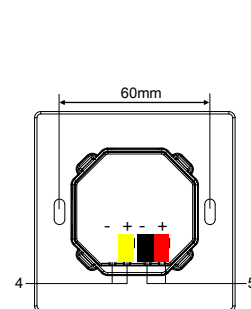
Figure 7. Dimensions - Back View (EU)
