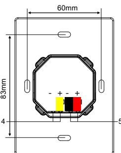
Figure 8. Dimensions - Back View (US)
