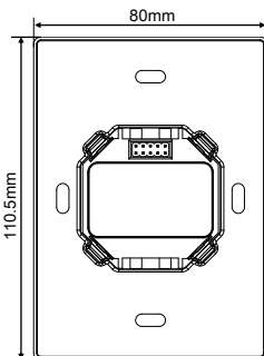
Figure 4. Dimensions - Front View (US)
