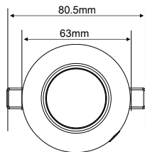
Figure 2. Dimensions - Front View
