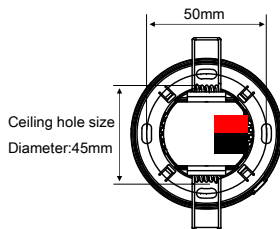
Figure 4. Dimensions - Back View
