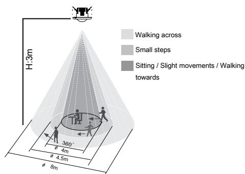
Detection Range (25°C)
