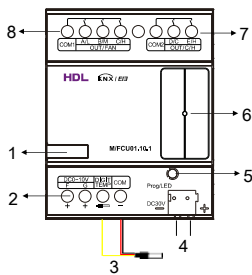
Figure 4. Components
