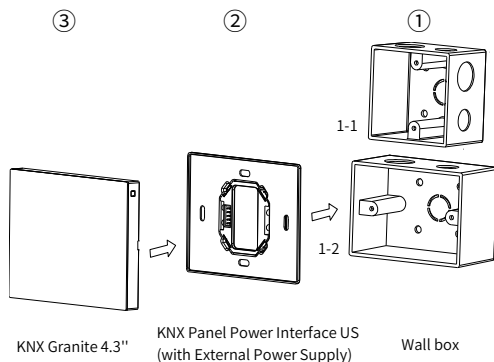
Figure 10. Landscape Installation
