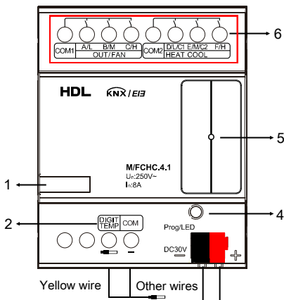
Figure 5. Wiring
