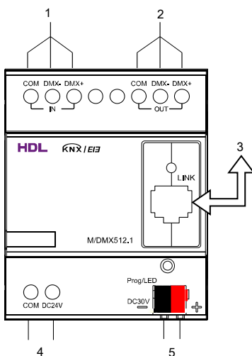
Figure 4. Wiring
