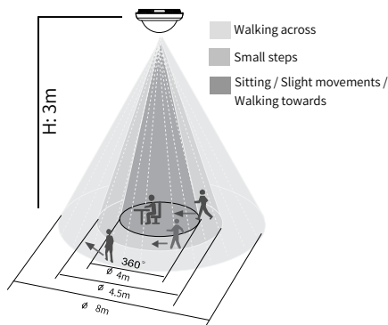
Detection Range (At 25°C)
