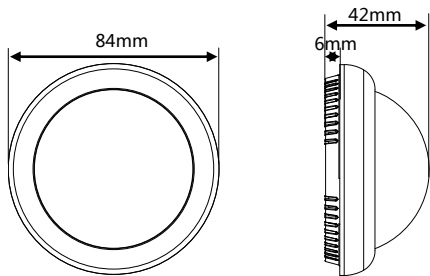
Figure 2. Dimensions - Front View Figure 3. Dimensions - Side View
