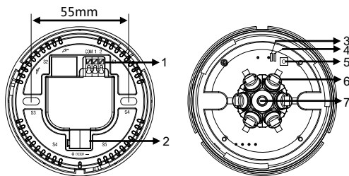
Figure 4. Dimensions - Back View Figure 5. Components - Interior View
