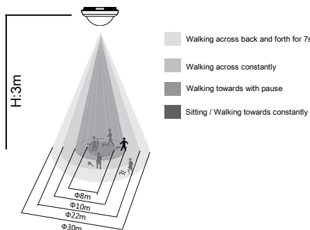
Detection Range (At 29°C)
