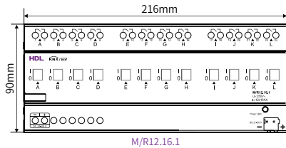
Figure 6. Dimensions - Front View
