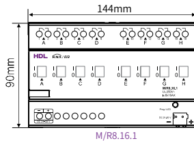
Figure 5. Dimensions - Front View
