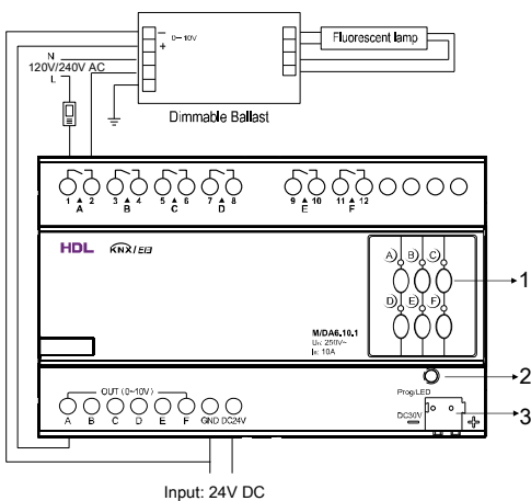
Figure 4. Wiring
