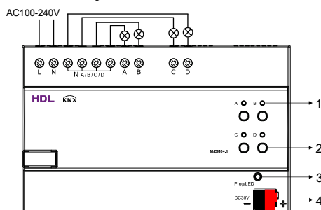
Figure 8. Wiring
