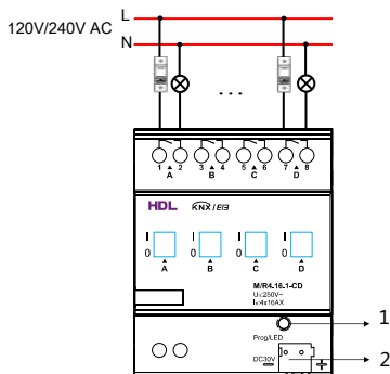
Figure 8. Wiring
