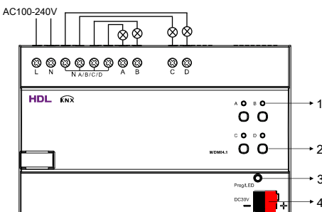
Figure 8. Wiring
