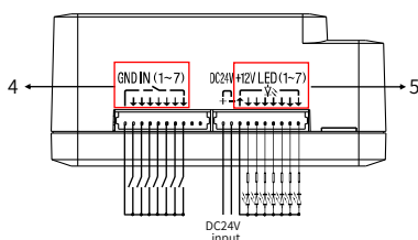
Figure 5. Wiring
