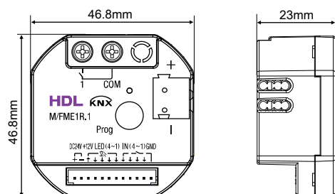
Figure 3. Dimensions - Front View Figure 4. Dimensions - Side View 1CH 16A Flush-mounted Switching Actuator (EU)
