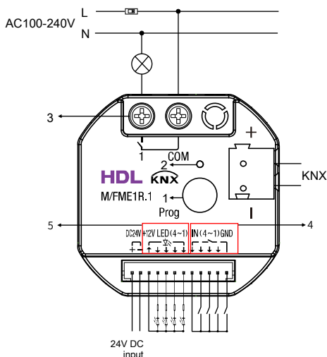
Take the connection of M/FME1R.1 as an example
