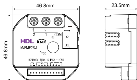
Figure 5. Dimensions - Front View Figure 6. Dimensions - Side View 2CH 10A Flush-mounted Switching Actuator (EU)
