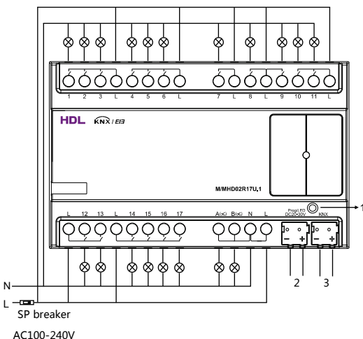
Figure 4. Wiring
