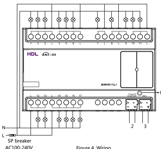
Figure 4. Wiring
