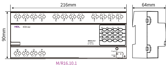
Figure 8. Dimensions - Front View
