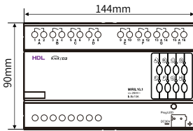
Figure 6. Dimensions - Front View
