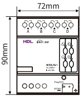
Figure 5. Dimensions - Front View
