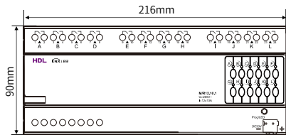
Figure 7. Dimensions - Front View
