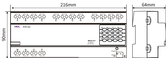
Figure 8. Dimensions - Front View Figure 9. Dimensions - Side View
