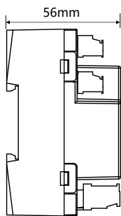
Figure 3. Dimensions - Side View
