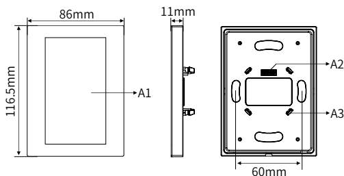
Figure 2. Dimensions - Front View
