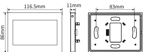
Figure 6. Dimensions - Front View
