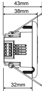
Figure 3. Dimensions - Side View
