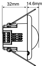
Figure 3. Dimensions-Side View
