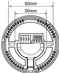
Figure 3. Dimensions-Back View
