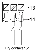
Figure 7. Dry contact wiring
