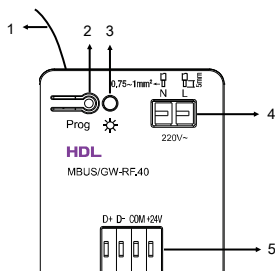
Figure 5. Components
