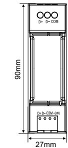
Figure 5. Base - Front View
