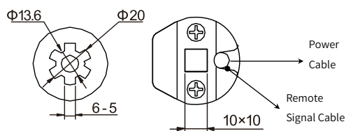
Figure 5. Dimensions—Motor Bottom View (Unit: mm)
