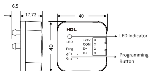
Figure 3. Dimensions—Communication Module (Unit: mm)
