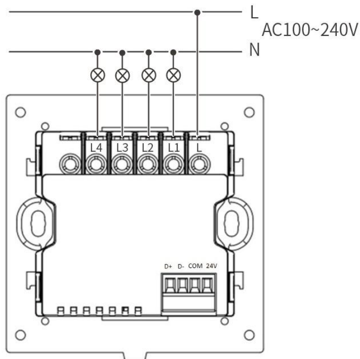
Panel power interface with 4CH relay
