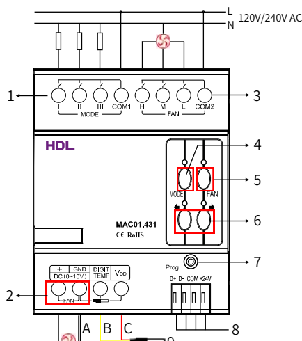
Figure 4. Wiring
