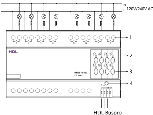
Figure 4. Wiring
