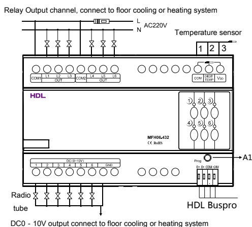
Figure 4. Wiring
