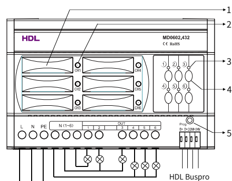
Figure 4. Wiring
