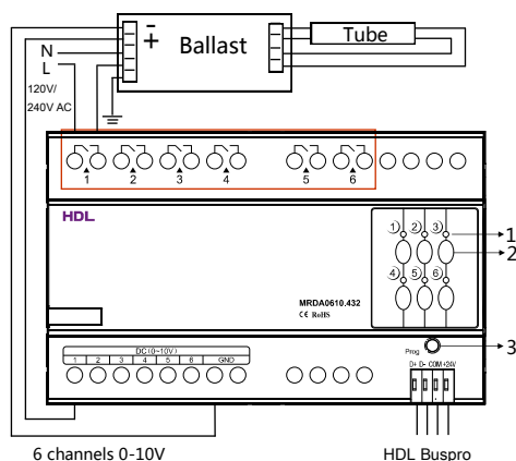
Figure 4. Wiring
