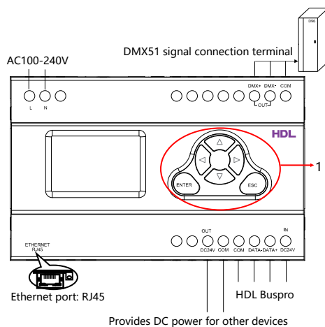
Figure 4. Wiring
