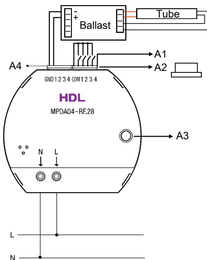
Figure 4. Wiring
