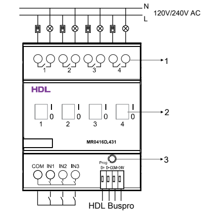
Take the connection of HDL-MR0416D.431 as an example Figure 8. Wiring
